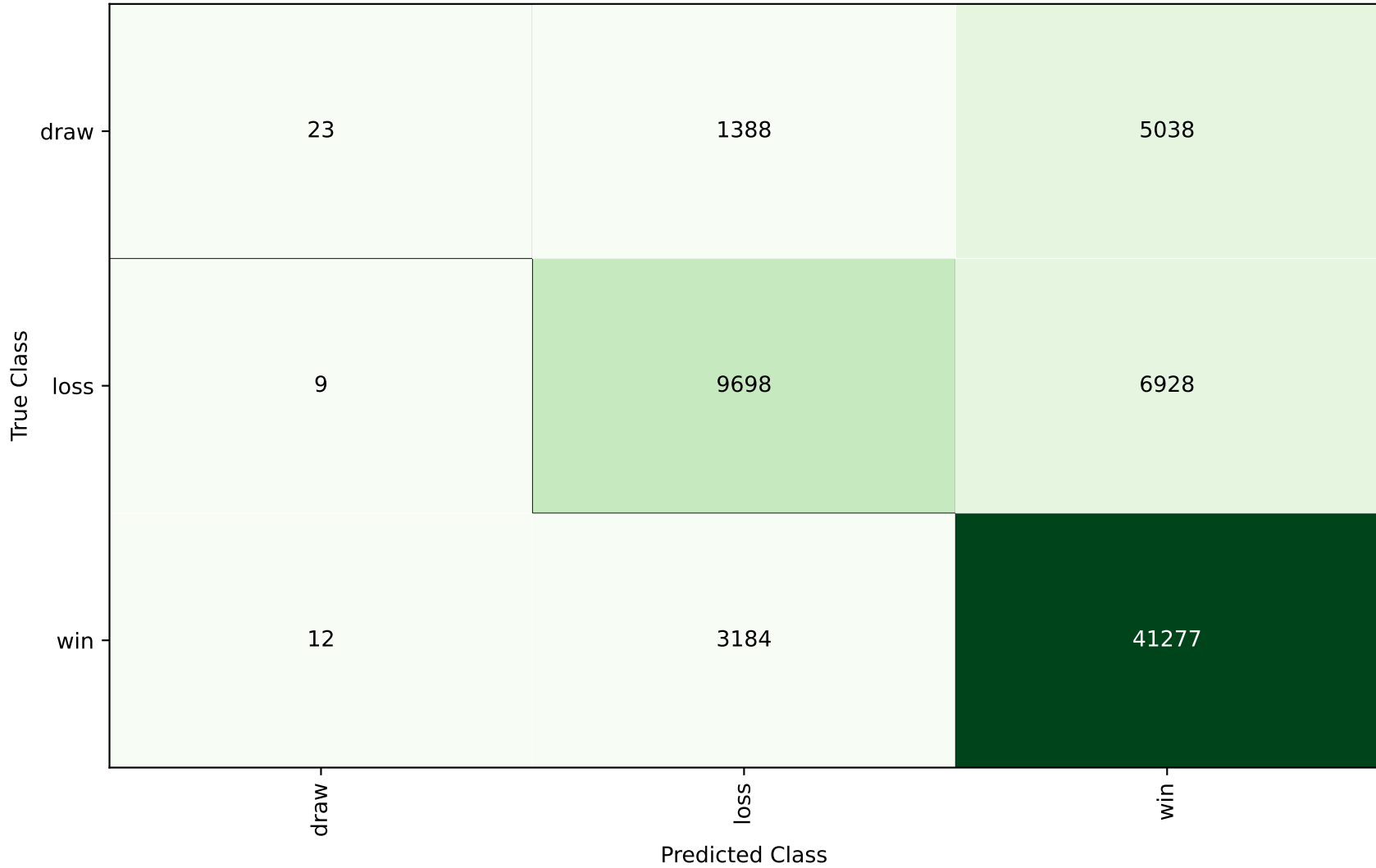
RidgeClassifier Confusion Matrix
